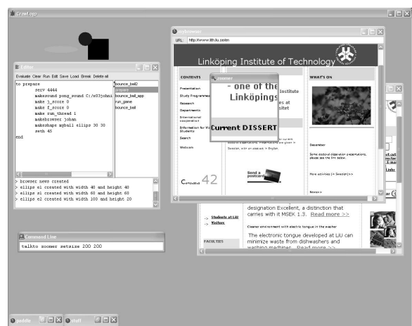
Figure 2: CrawLogo workspace
